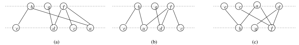
Figure 1: A tree and three different embeddings of the tree on 2 levels.
